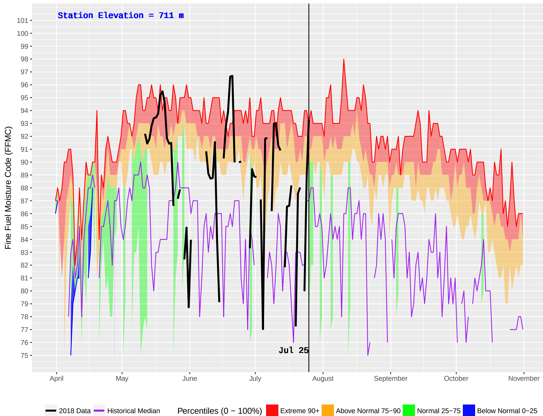
TOAD RIVER (126) : Historical (1981–2016) and Current (2018) Noon Fine Fuel Moisture Code (FFMC)
